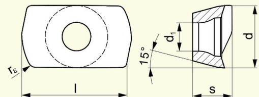
ADEX HF
