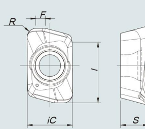
XPET
